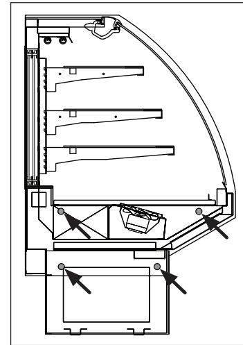
Fig. 5 Bolt locations (SMD-R CANDY)
