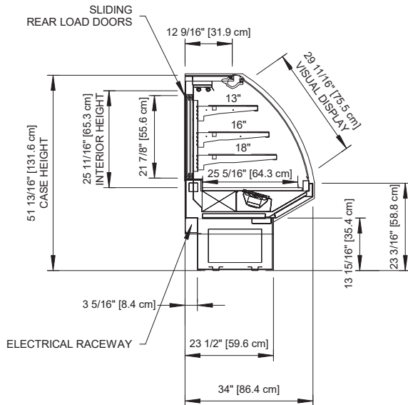
CURVED GLASS
