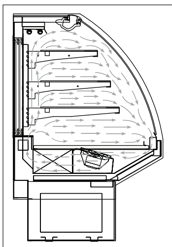
Fig. 15 Airflow pattern (SMD-R CANDY)
