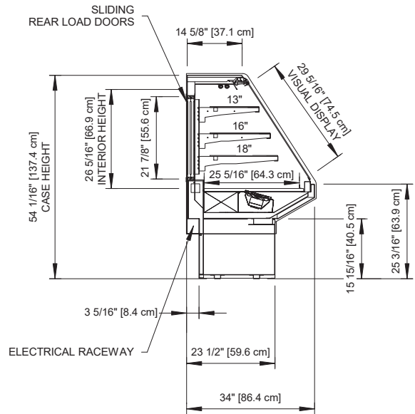
FLAT GLASS (OPTIONAL)
