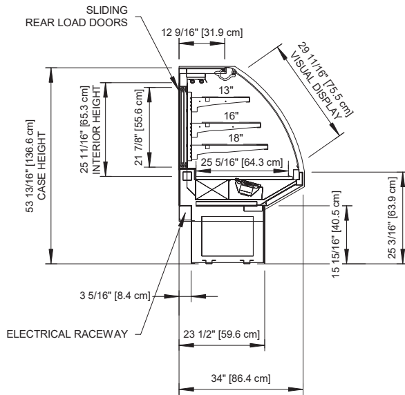
CURVED GLASS
