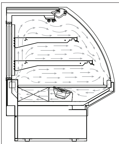
Fig. 14 Airflow pattern (SMD-R BAKERY)
