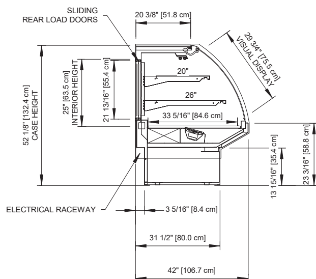
CURVED GLASS
